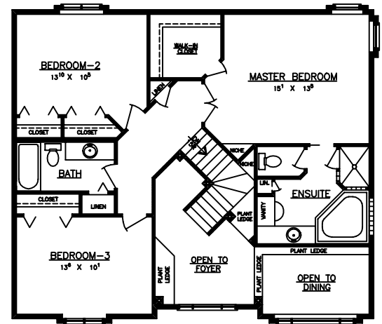
SECOND FLOOR AREA = 928 S.F.
